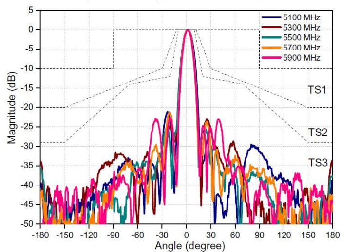
V-plane Co-polarization Pattern
